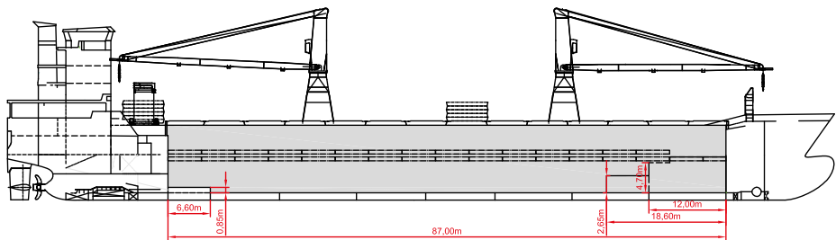
SIDE VIEW
