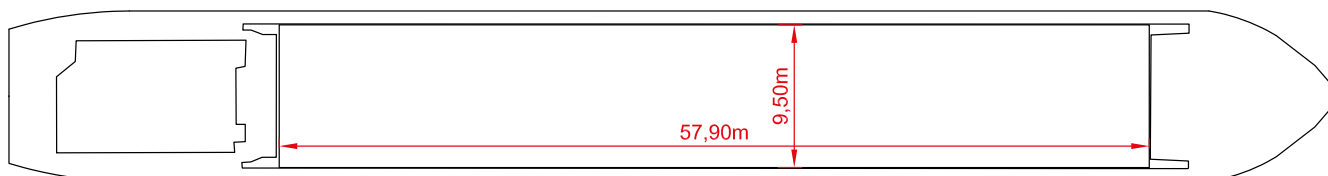
Main Deck
